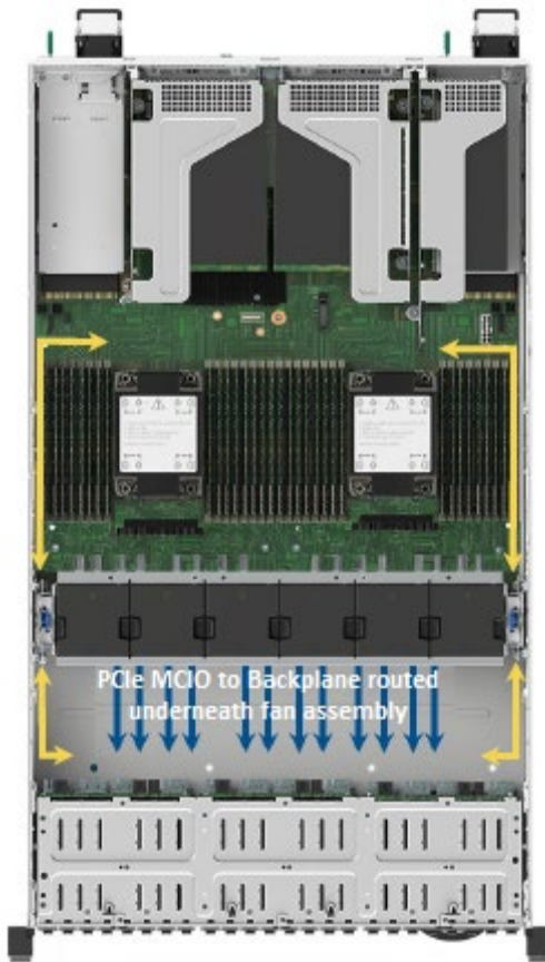
2U Server System Cable Routing
