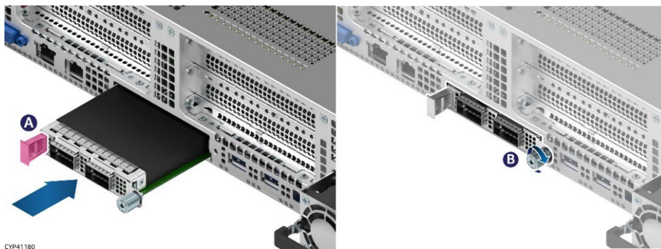
Figure 30. OCP* Module with Pull Tab Installation (2U System Shown)
