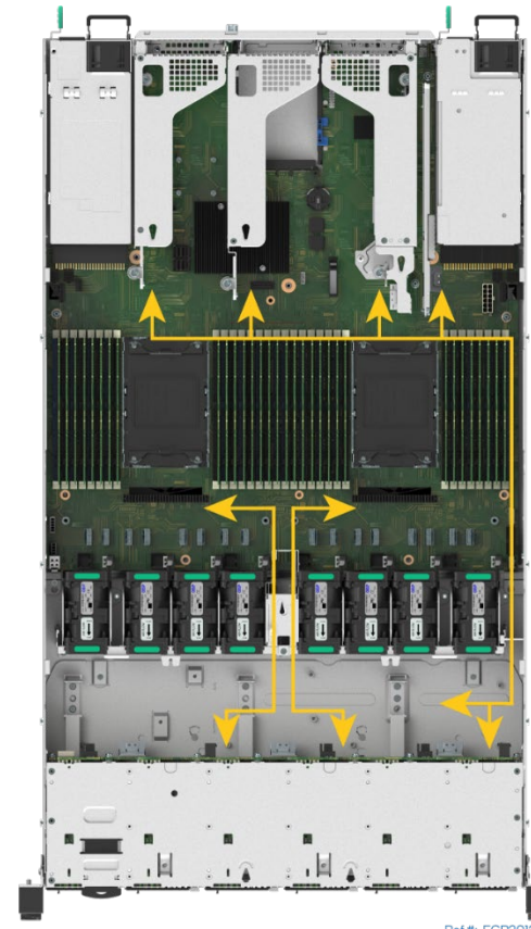
1U Server System Cable Routing
