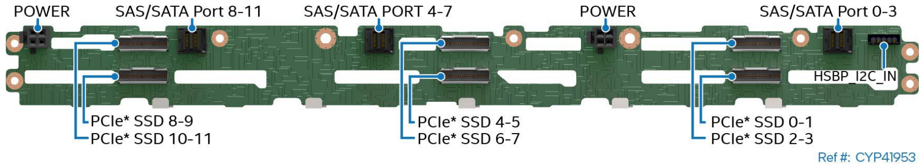
Figure 19. 1U 12 x 2.5" SAS / SATA / NVMe* Hot Swap Backplane – Back Side
